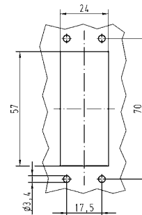
Assembly cut out bulkhead mounted housing 57 x 24 mm
