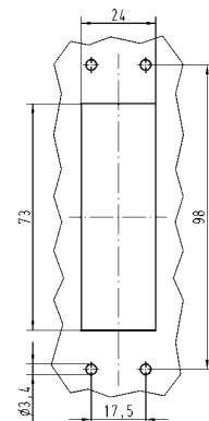
Assembly cut out bulkhead mounted housing 73 x 24 mm
